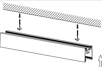
Tak installation
