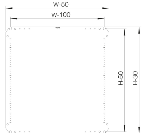
Mounting plate view
