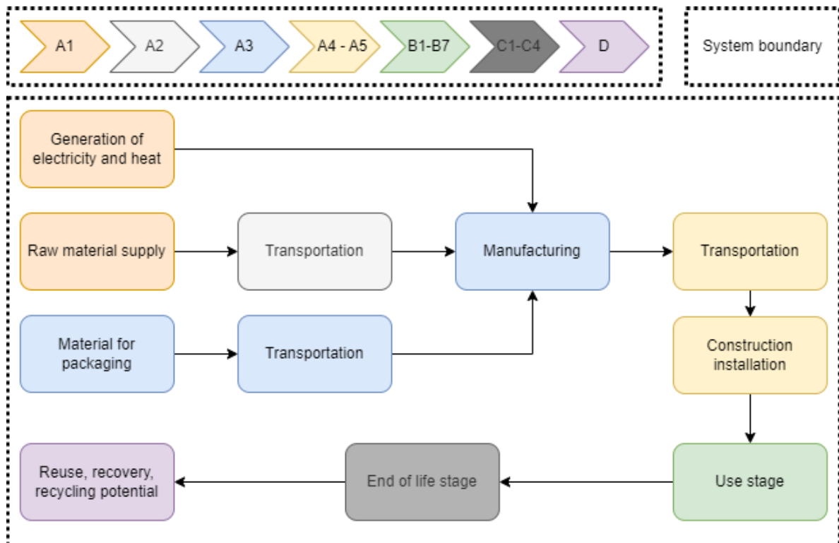
Figure 1 System boundary of the LCA study conducted on production of LILY
