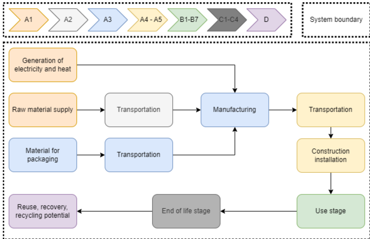
Figure 1 System boundary of the LCA study conducted on production of MIRA FL S
